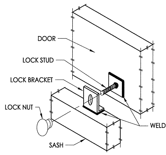
SASH LOCK DETAIL OPTIONAL
