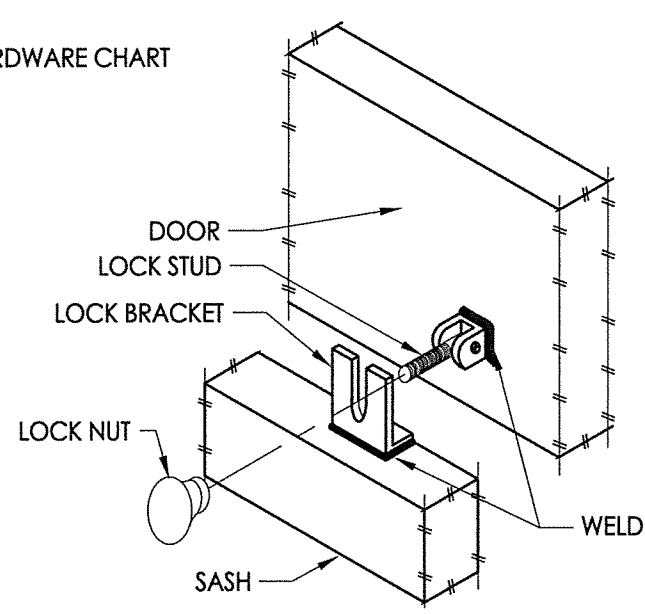
CAM LOCK DETAIL
