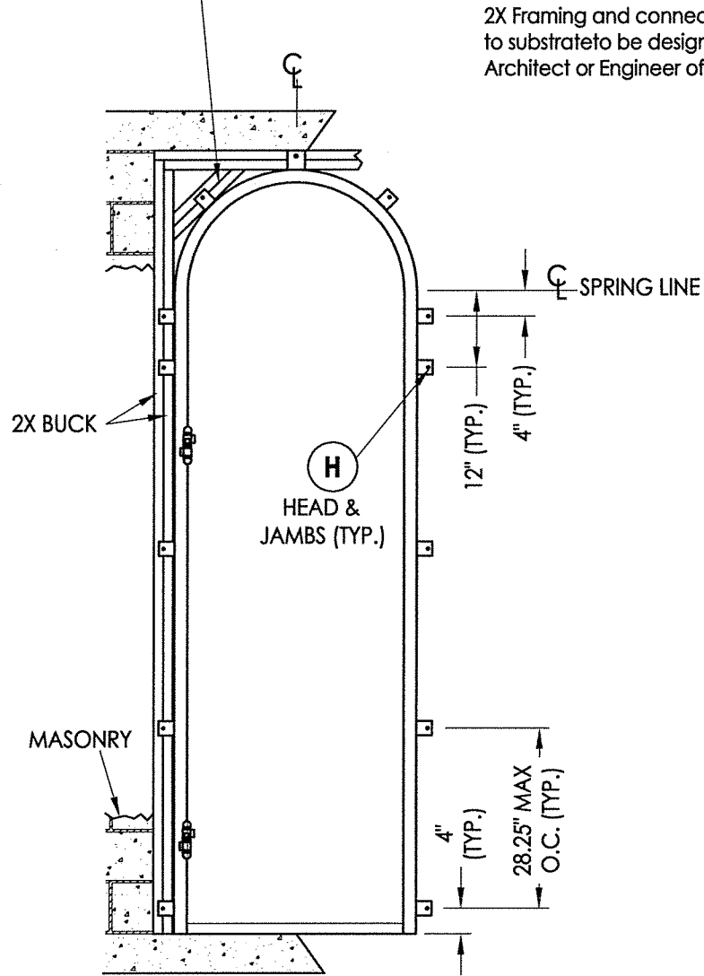
FRAME ANCHORING Stud Construction
