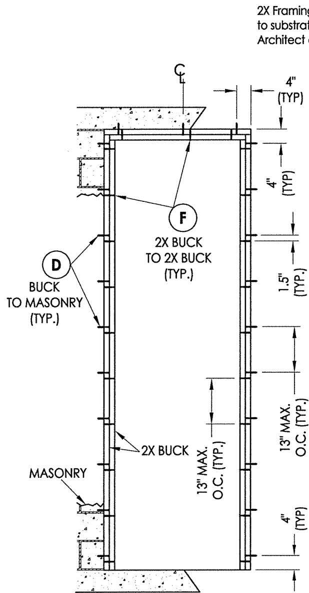
BUCK ANCHORING Double Buck Shown (Single Buck Similar)
